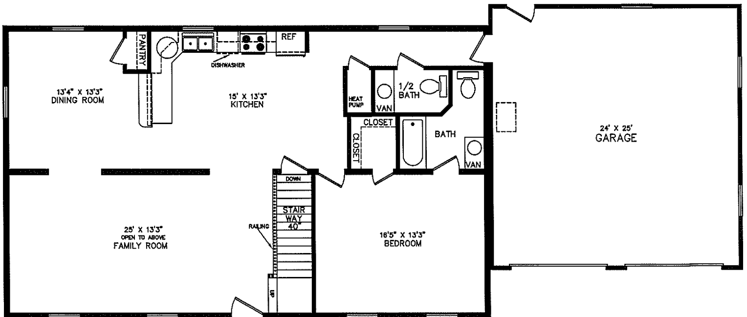
1st FLOOR
