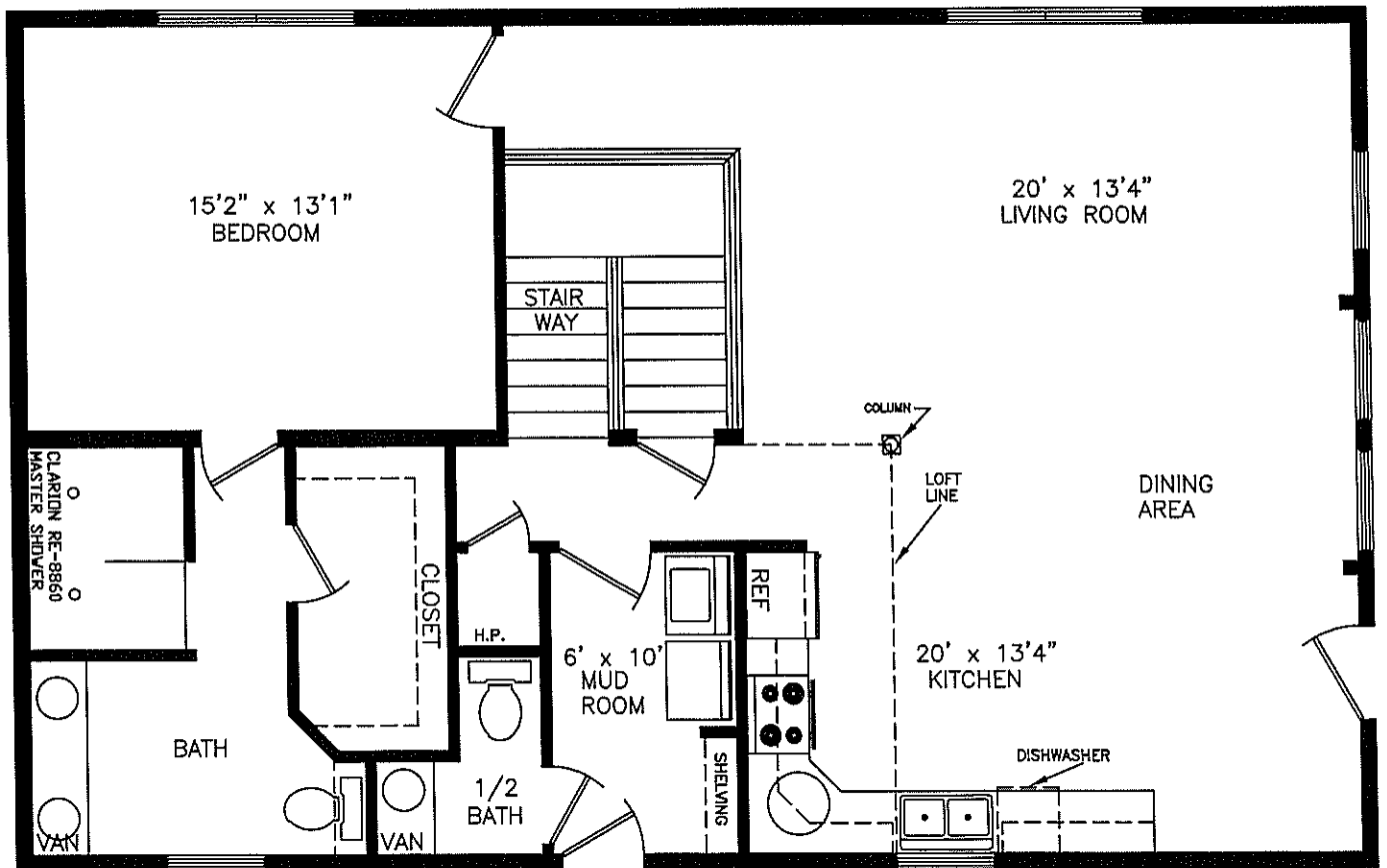
1st FLOOR
