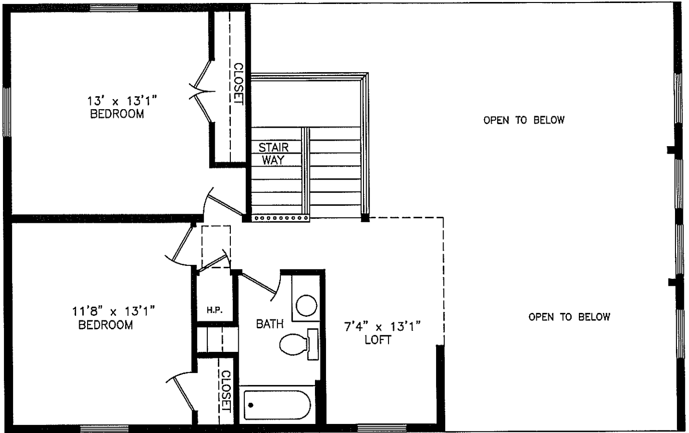
2nd FLOOR
